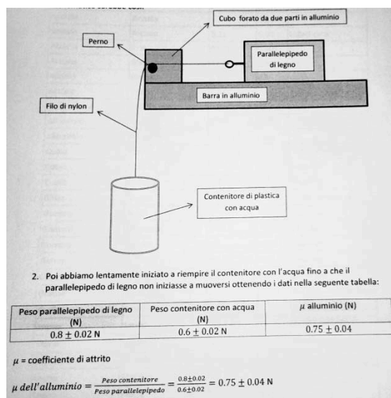
Figure 2. A schematic draw of a quantitative measurement of the static friction.
