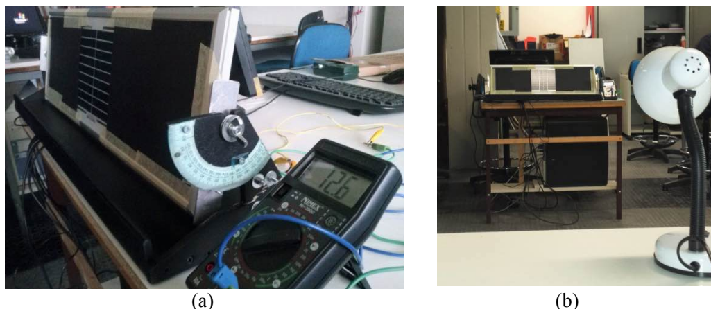
Figure 2. Experimental setting used for the measurement of the light flow on a solar panel according to (a) the incident angle, (b) the distance between the source and the panel. The sensible area of the panel is about 200 \text{ cm}^2 , the distance between the light lamp and the center of the panel ranges from 120 to 310 cm.
