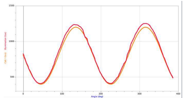
Figure 9. Graphs of the data collected with the apparatus in Figure 8, and an \text{Acos}^2\theta model for Intensity vs. Angle.
