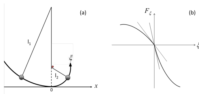
Figure 4. (a) An interrupted pendulum. (b) Graph of the \zeta -component of the restoring force, F_\zeta , vs \zeta .
