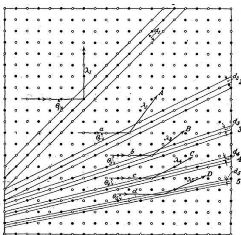
Figure 3. Schematic representation of the reflection by a crystal of rock salt (NaCl) of an heterochromatic X-rays incident beam (Richtmyer, F.K. (1934). Introduction to modern physics , 2 nd edition, McGraw-Hill, New York)
