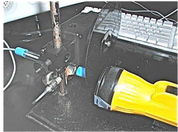
Figure 8. Computer-based apparatus used to analyze polarized light.
