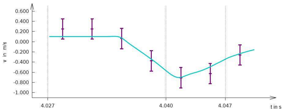
Figure 4. Comparison of velocity-time-diagrams. Purple dots, with error bars: calculated data from video. Turquoise curve: calculation from acceleration data of sensor
