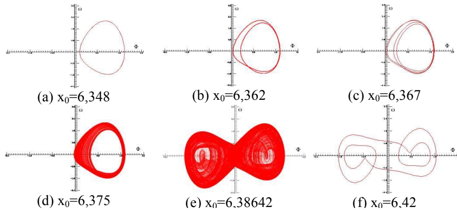
Figure 3: The trajectories of motion in phase plane with (\Phi_0 = 0, \omega_0 = 0, \Theta_0 = 0)
