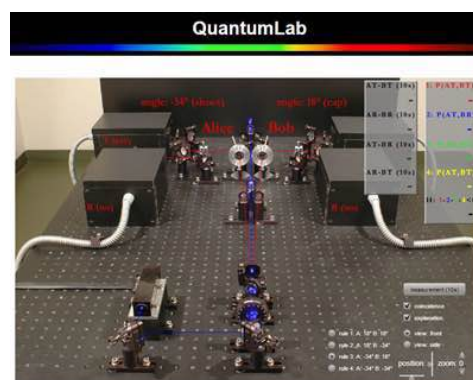
Figure 12. QuantumLab Entanglement & Non-locality
