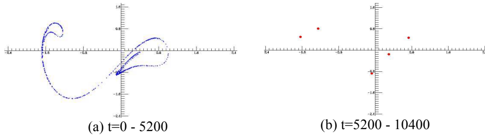
Figure 7: Stroboscopic map of the transient chaos
